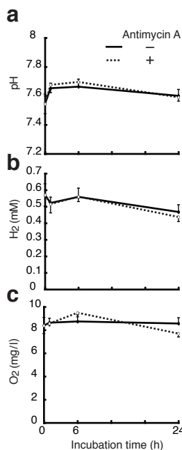
Supplementary Figure 2 pH, \text{H}_2 and \text{O}_2 maintain constant in culture medium in a closed flask filled with a mixed gas.
